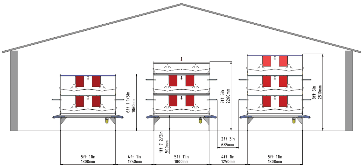
Example of two and three tier nest layout
